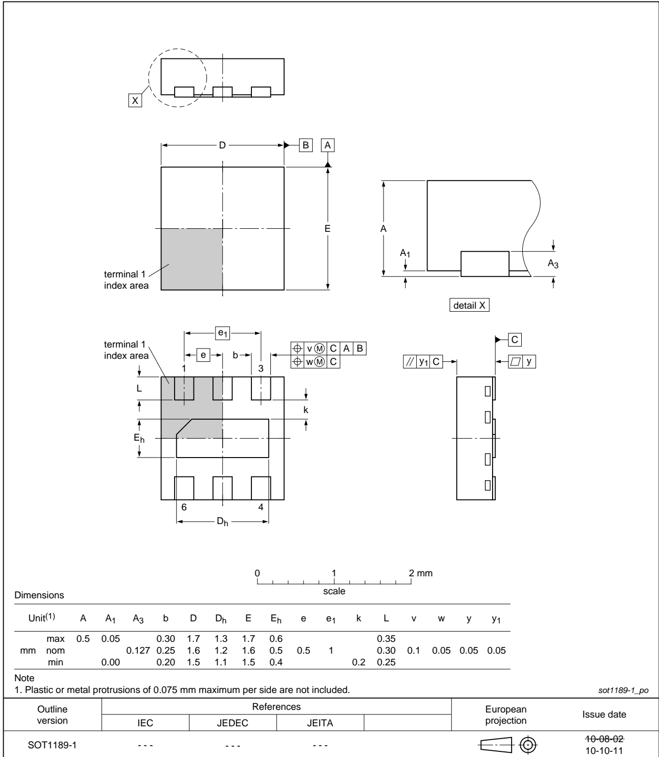
Fig 4. Package outline DFN1616-6 (SOT1189-1/XSON6)
